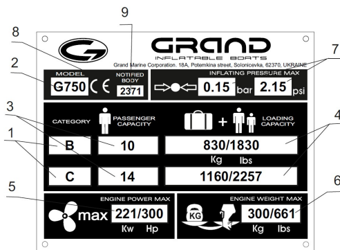
Fig. 15. Builder's plate.
