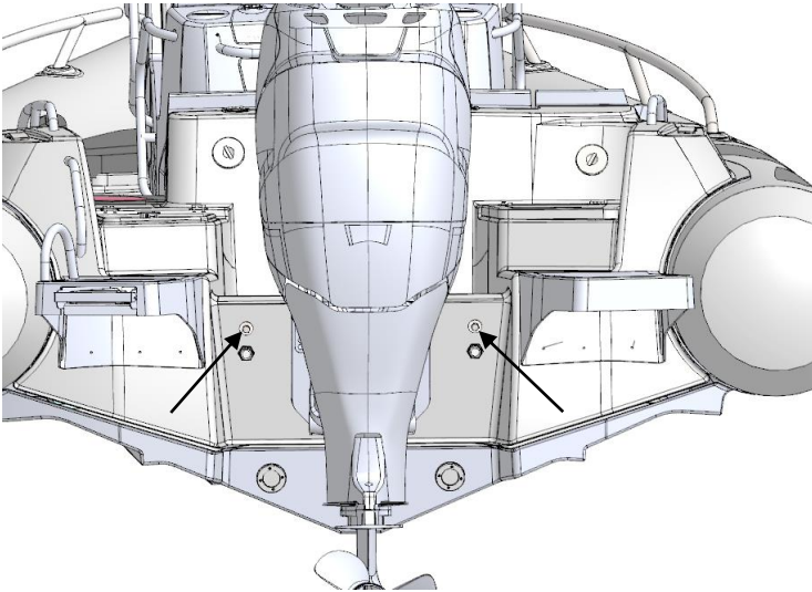
Fig. 6. Recess drainage.
