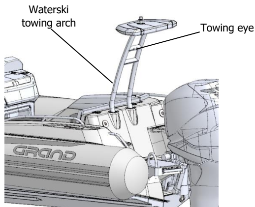
Fig. 42. Waterski towing arch.
